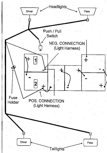
Club Car Basic 36-Volt Wiring Diagram
